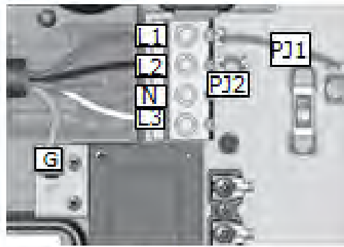
3-phase with single neutral
