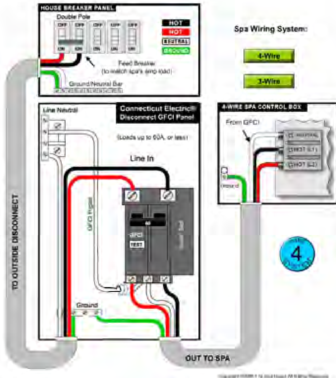
Figure 2. GFCI Wiring Schematic for 60 Hz Systems
